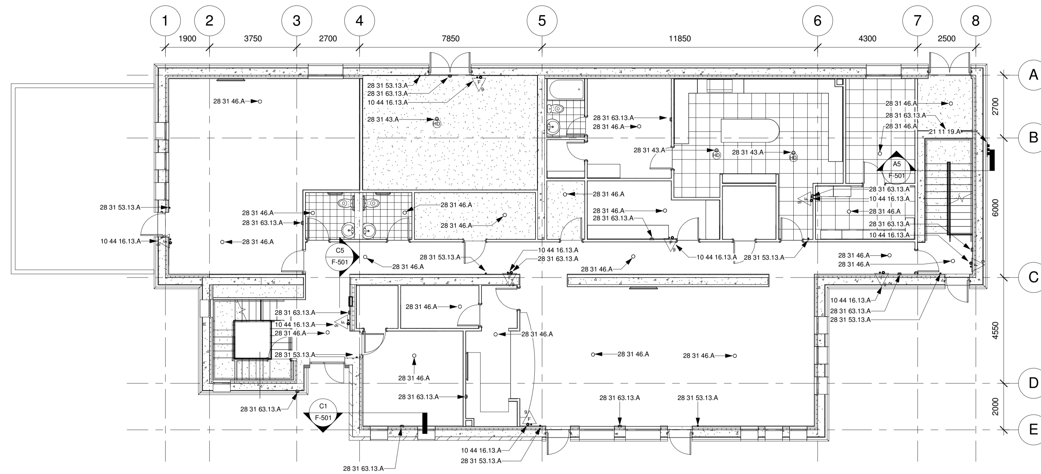
C2 Level 1-Fire Alarm System 1 : 100
