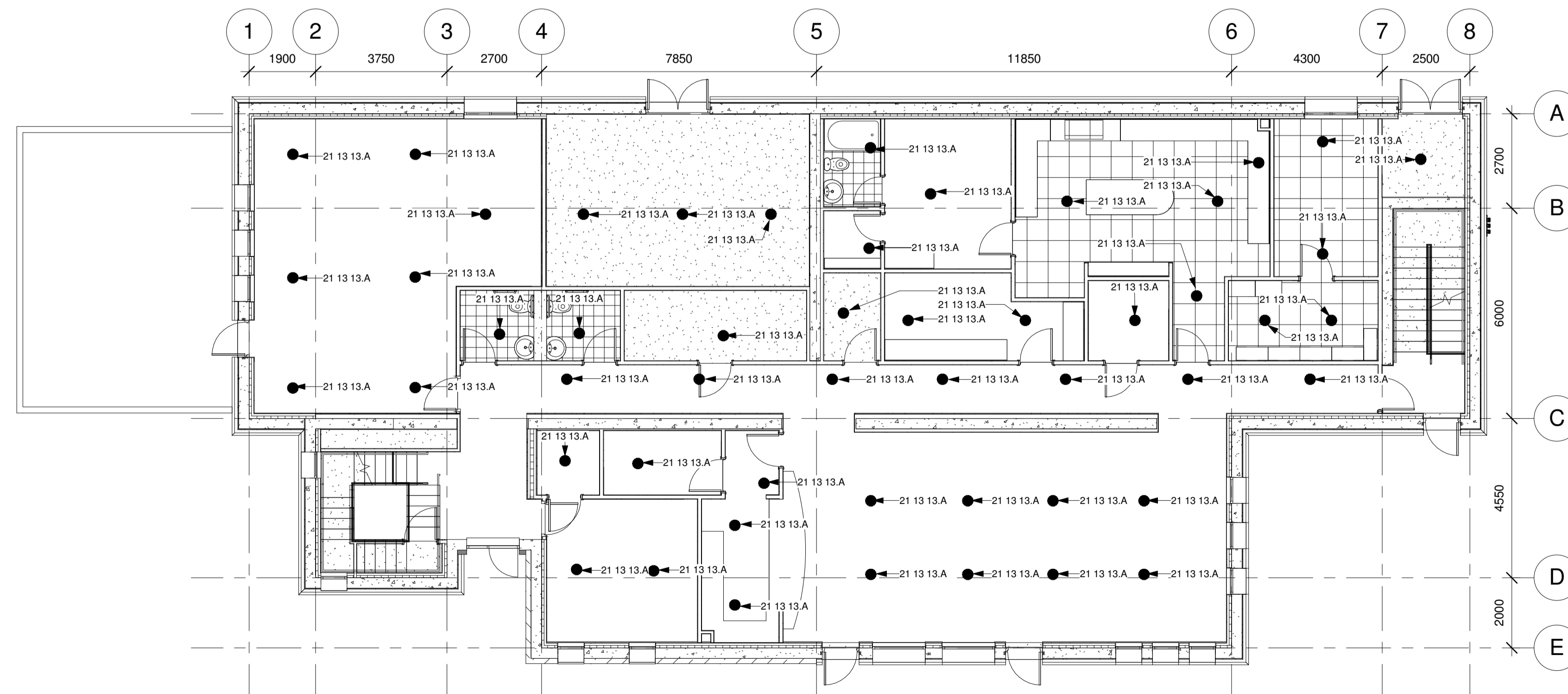
A2 Level 1-Sprinkler System 1 : 100
