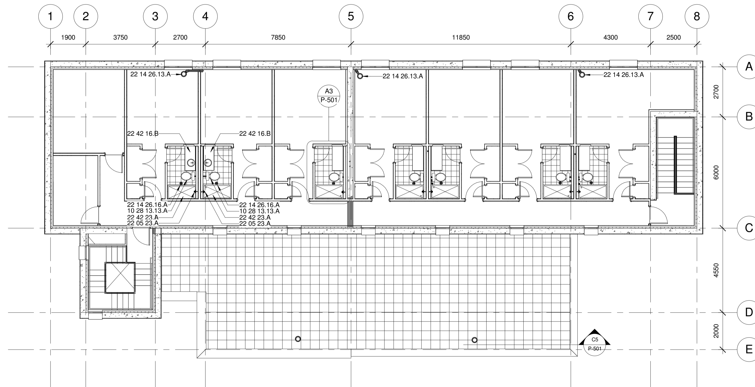
Level 2 - Full Height 1 : 100
