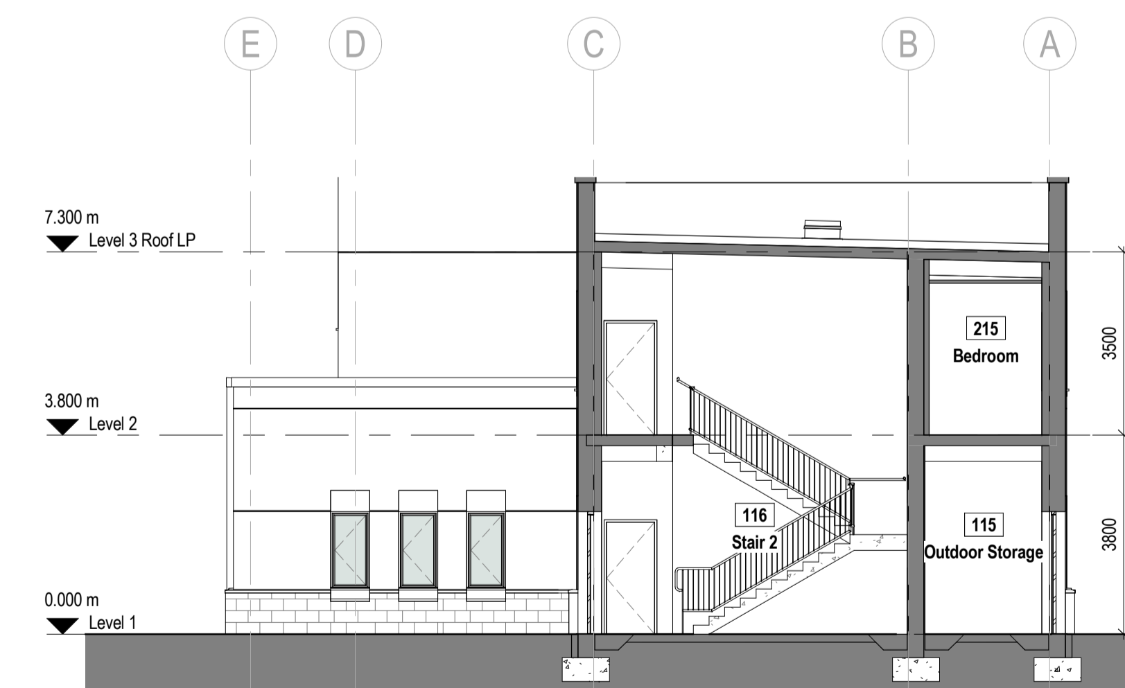
D Building Section DD
