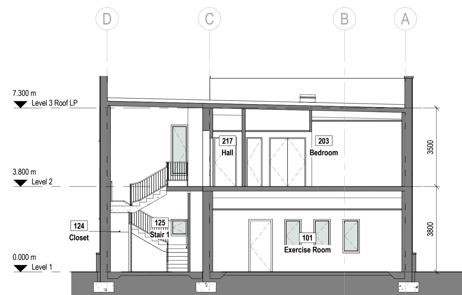
C Building Section CC
