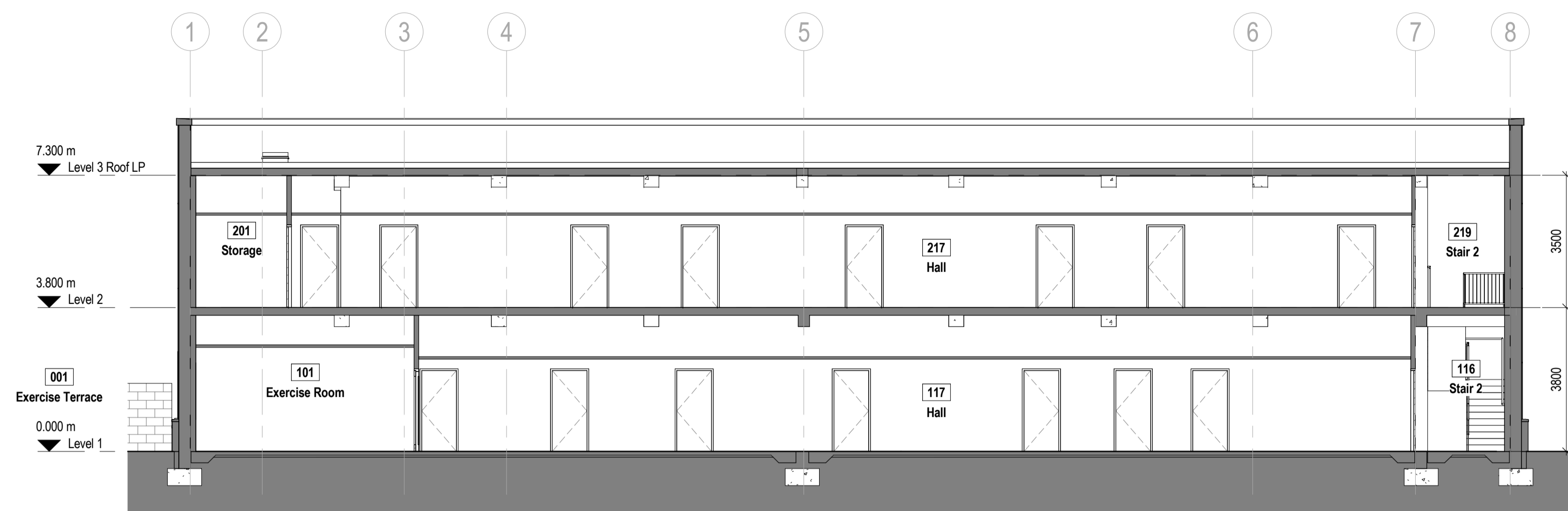
A Building Section AA
