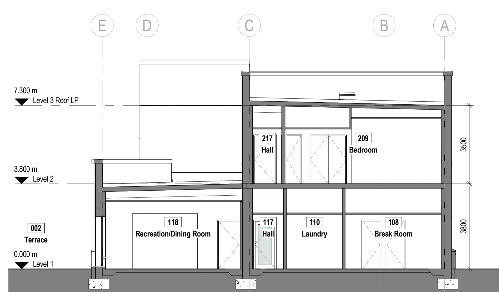
B Building Section BB
